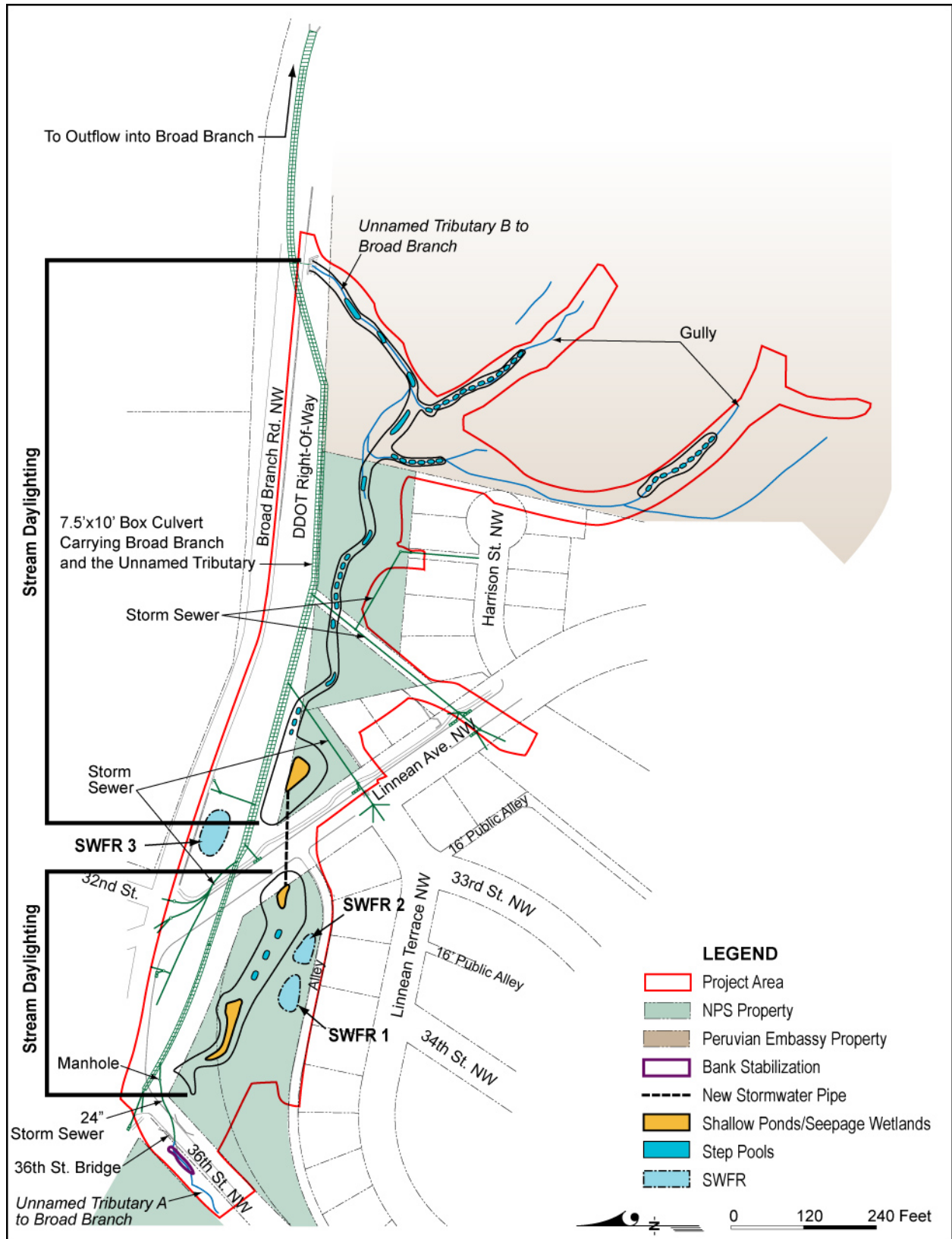
Figure 4: Alternative 2 - Full Restoration
