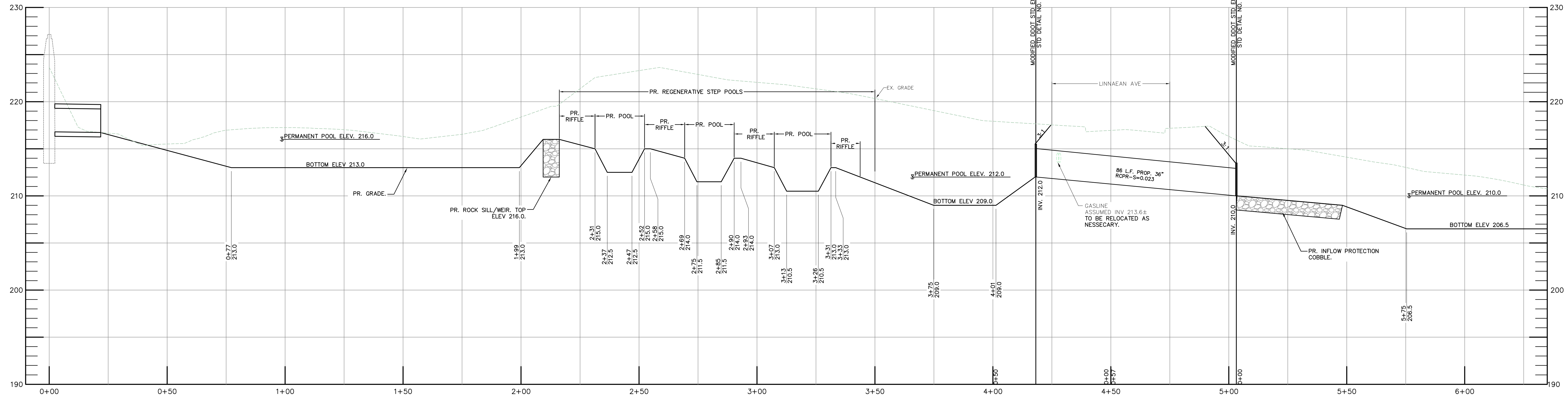
PROFILE PR C/L BROAD BRANCH 0+00 TO 6+25 SCALE: HORIZONTAL 1" = 20' VERTICAL 1" = 5'
